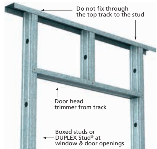
DETAIL A: DOOR/WINDOW HEAD DETAIL
