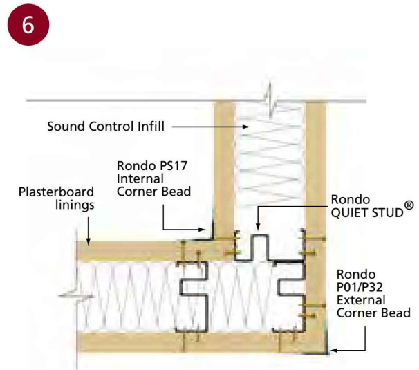
■ CORNER DETAIL
