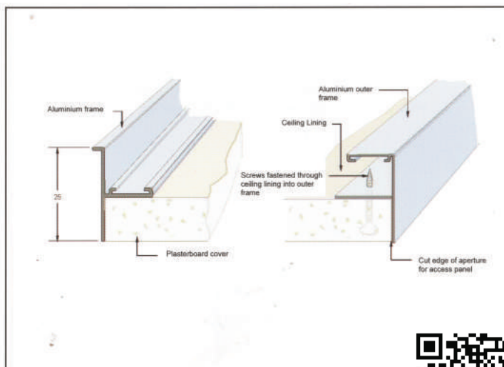
ACCESS PANEL – Framing profiles
