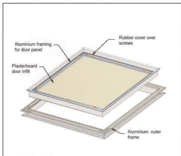
ACCESS PANEL – Push up and slide panel
